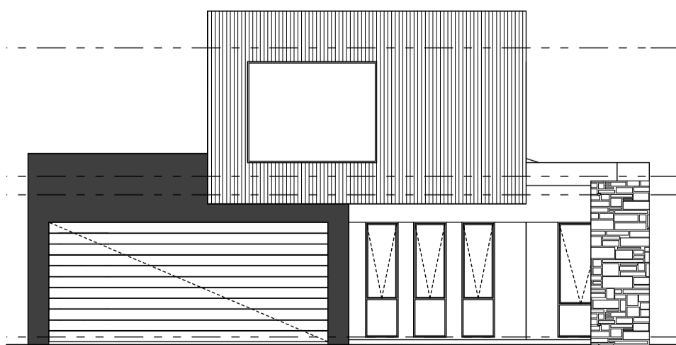
FRONT ELEVATION
