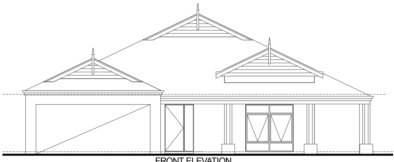
FRONT ELEVATION
